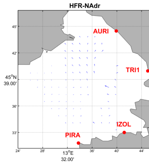
Map of the HFR-NAdr network area. Red dots indicate the position of the sites
