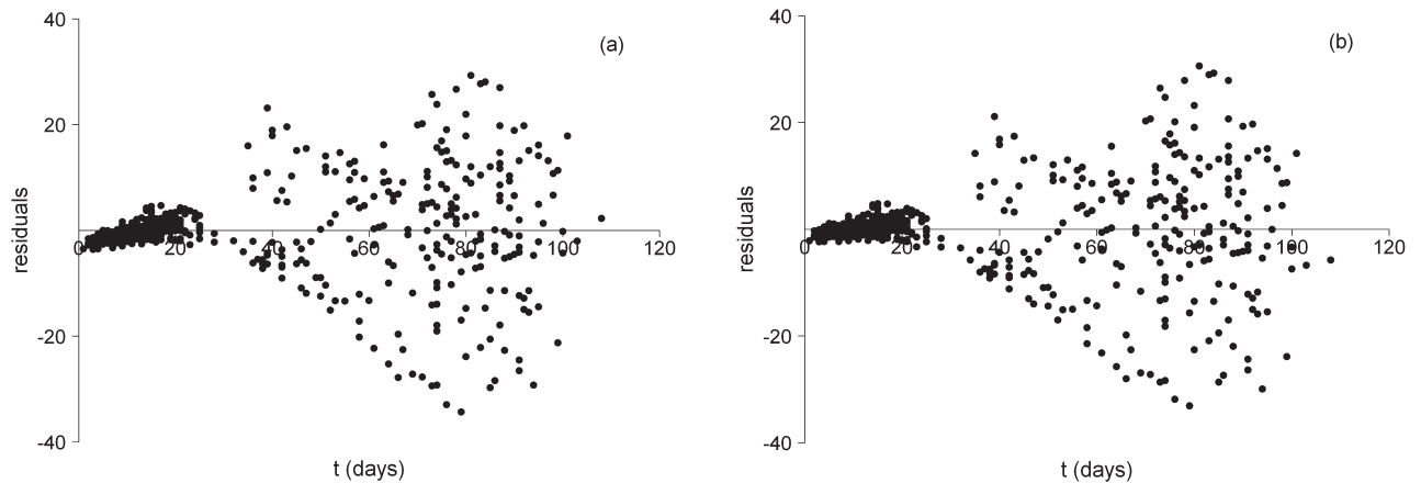
FIG. 2. – Plots of standard length residual values for (a) logistic and (b) Gompertz growth equations at age.
