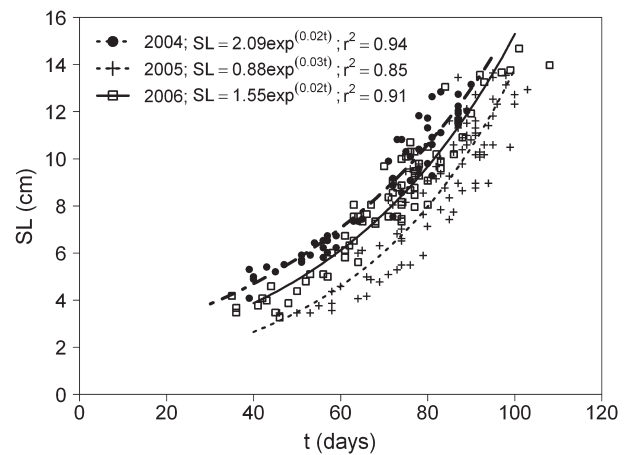
FIG. 4. – General growth pattern of juveniles sampled in different years. SL, standard length; t, age.
