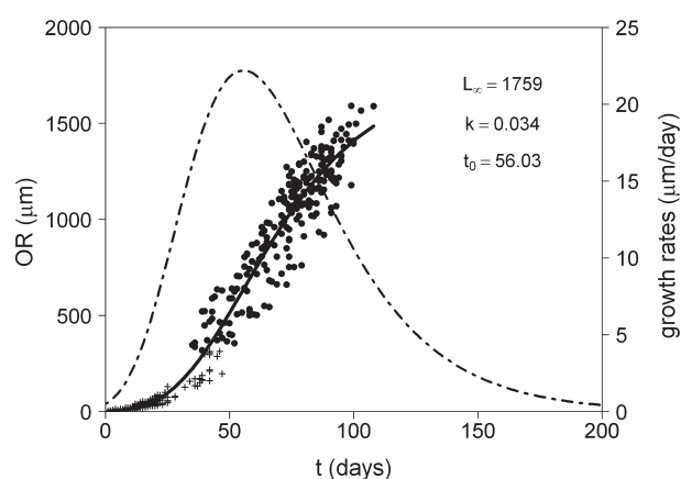
FIG. 7. – Gompertz curve (solid line) fitted to otolith radius (OR) at age (t) data. Daily growth increments (broken line) have also been plotted considering the difference in otolith radius between consecutive days obtained with the Gompertz curve. The crosses represent the larvae and the dots the juveniles. L_{\infty} , asymptotic otolith radius ( \mu\text{m} ); k , growth coefficient; t_0 , the abscissa of the inflection point (days).
