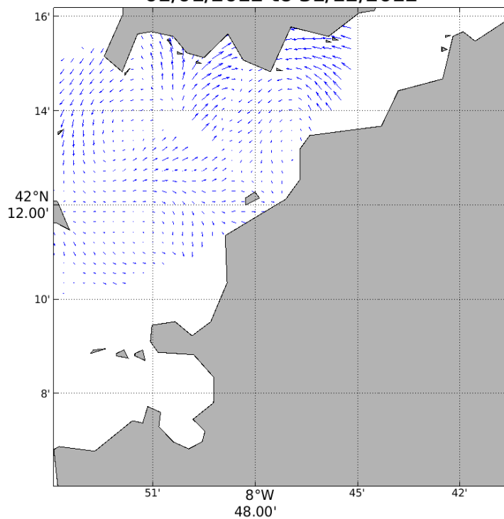
HFR-Vigo: HFR Surface current average [m/s] 01/01/2012 to 31/12/2012
