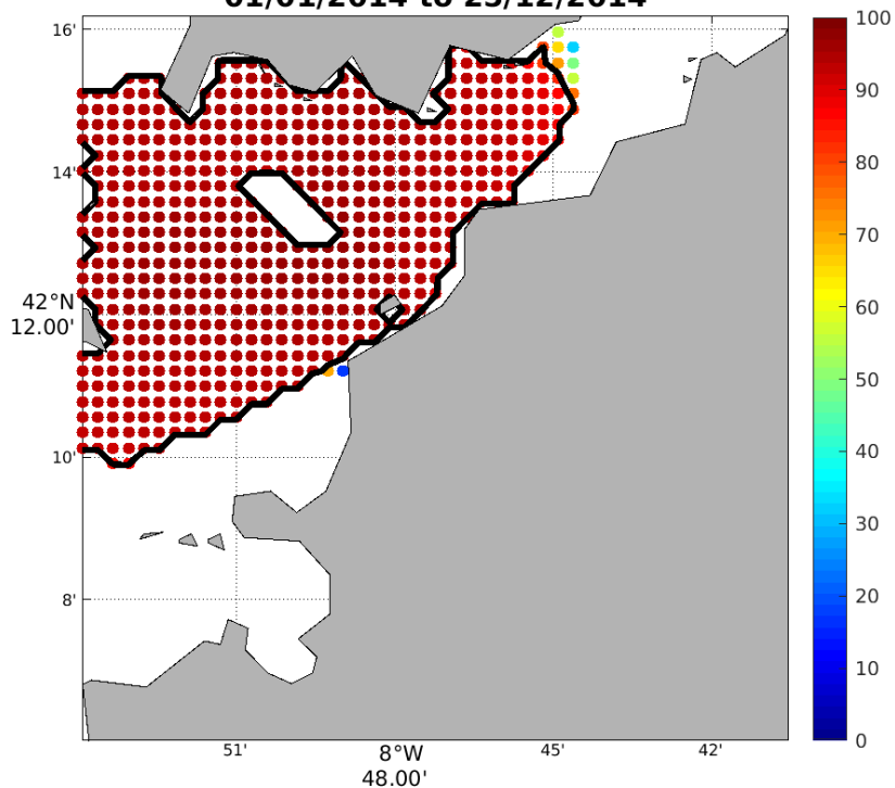
HFR-Vigo: Percent Total Vector Coverage (contour showing >80%) 01/01/2014 to 25/12/2014
