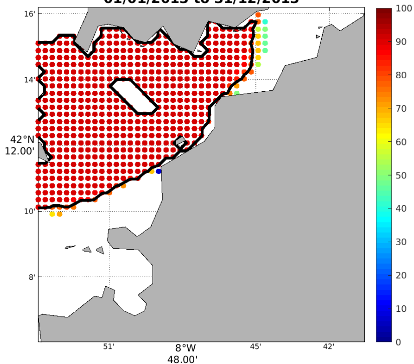
HFR-Vigo: Percent Total Vector Coverage (contour showing >80%) 01/01/2013 to 31/12/2013
