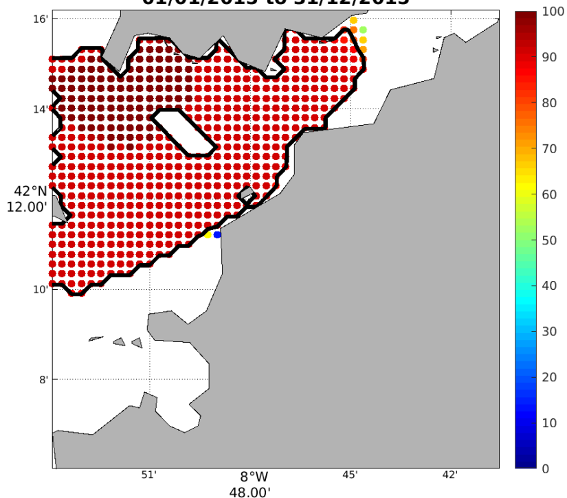
HFR-Vigo: Percent Total Vector Coverage (contour showing >80%) 01/01/2015 to 31/12/2015
