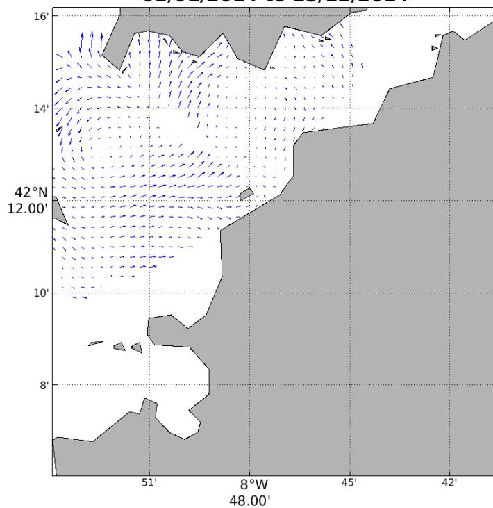
HFR-Vigo: HFR Surface current average [m/s] 01/01/2014 to 25/12/2014
